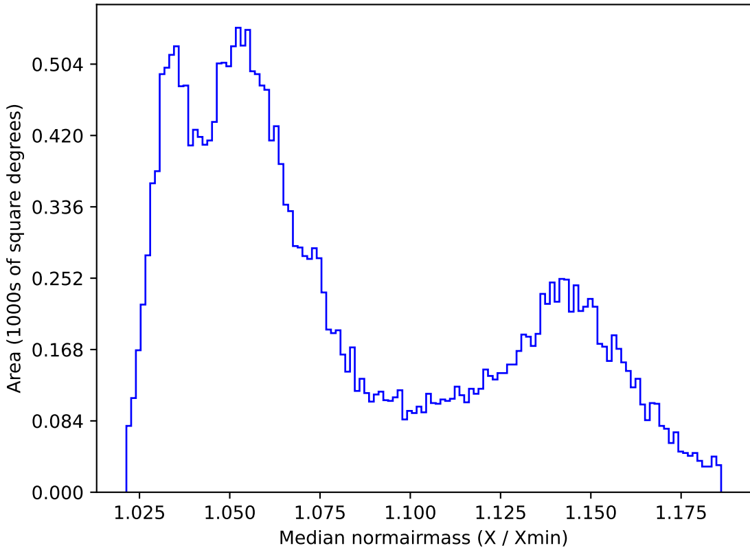
too_elab_heavy_r64_d2_gz_v3.4_10yrs All sky all bands: Median normairmass
