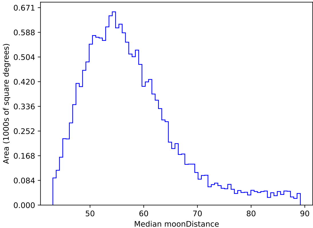
too_elab_heavy_r64_d2_gz_v3.4_10yrs WFD y band: Median moonDistance
