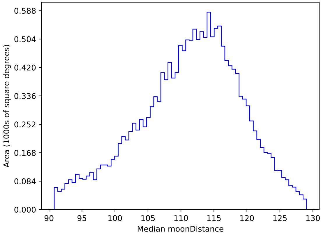
too_elab_heavy_r64_d2_gz_v3.4_10yrs WFD r band: Median moonDistance
