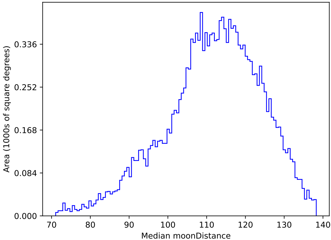
too_elab_heavy_r64_d2_gz_v3.4_10yrs WFD g band: Median moonDistance
