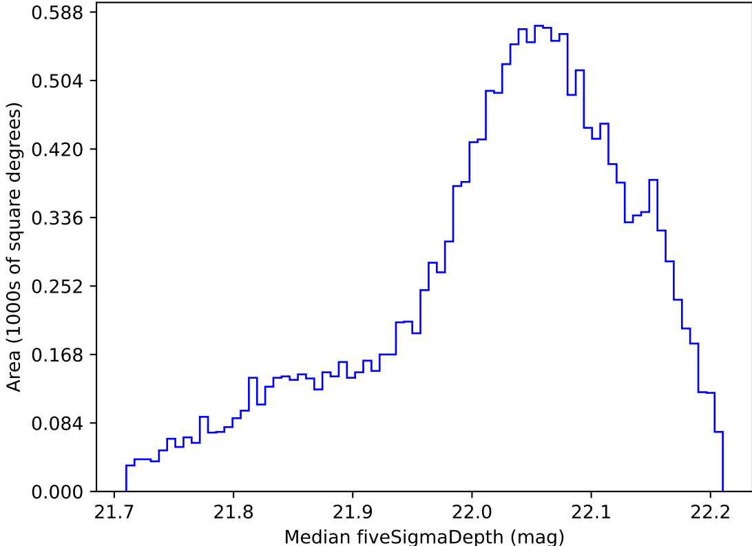
too_elab_heavy_r64_d2_gz_v3.4_10yrs WFD y band: Median fiveSigmaDepth
