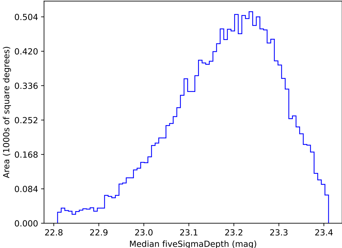
too_elab_heavy_r64_d2_gz_v3.4_10yrs WFD u band: Median fiveSigmaDepth
