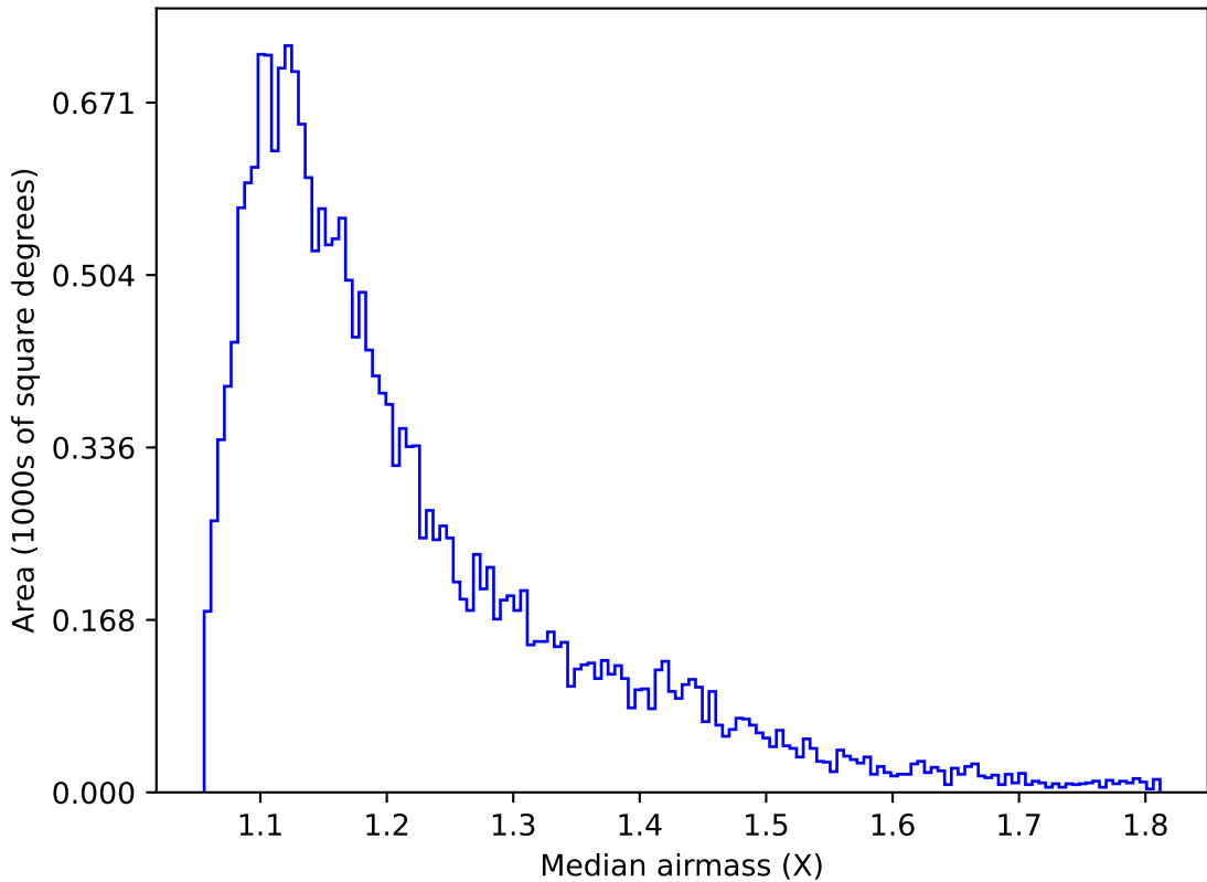
too_elab_heavy_r64_d2_gz_v3.4_10yrs Yr 1 u band: Median airmass
