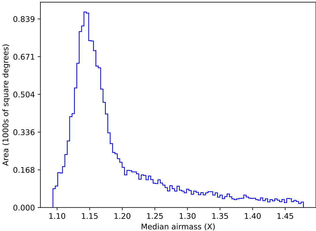
too_elab_heavy_r64_d2_gz_v3.4_10yrs WFD y band: Median airmass
