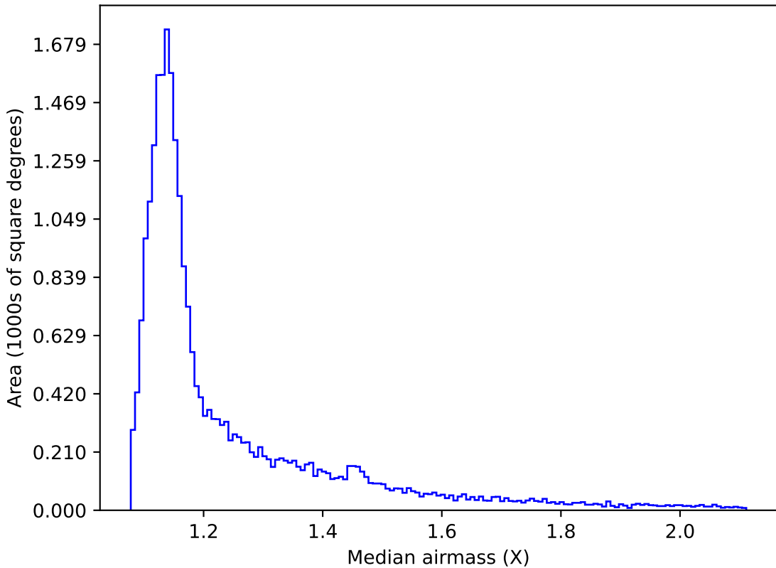
too_elab_heavy_r64_d2_gz_v3.4_10yrs All sky r band: Median airmass
