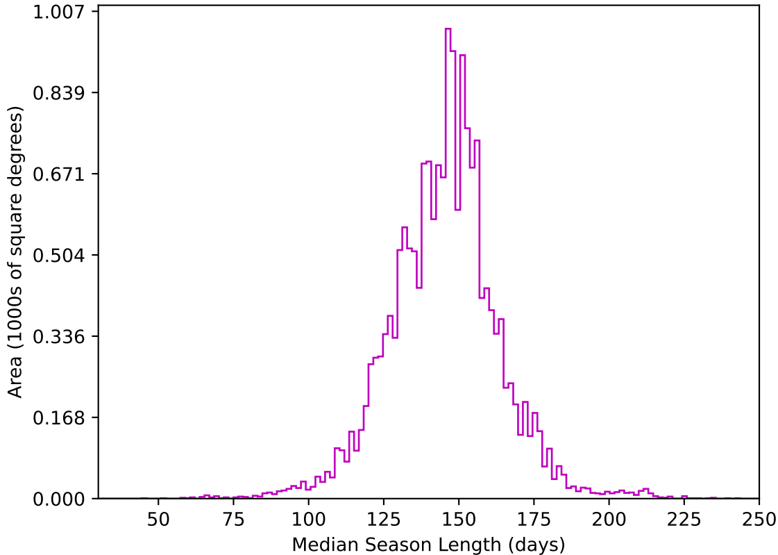
too_elab_heavy_r64_d2_gz_v3.4_10yrs WFD z band: Median Season Length
