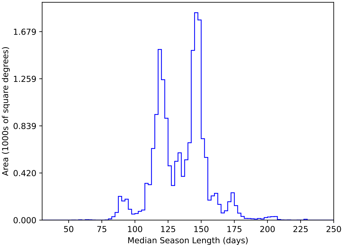
too_elab_heavy_r64_d2_gz_v3.4_10yrs WFD y band: Median Season Length
