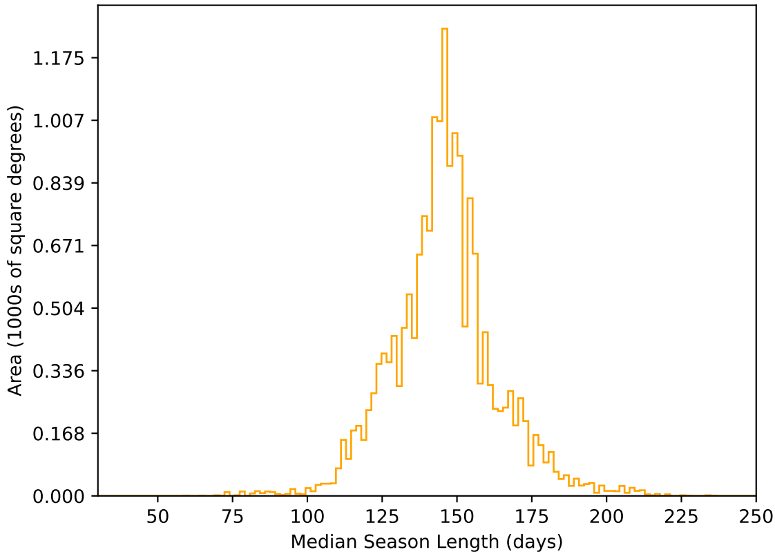
too_elab_heavy_r64_d2_gz_v3.4_10yrs WFD r band: Median Season Length
