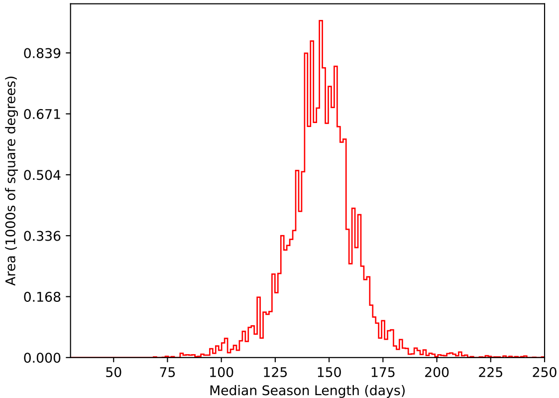
too_elab_heavy_r64_d2_gz_v3.4_10yrs WFD i band: Median Season Length
