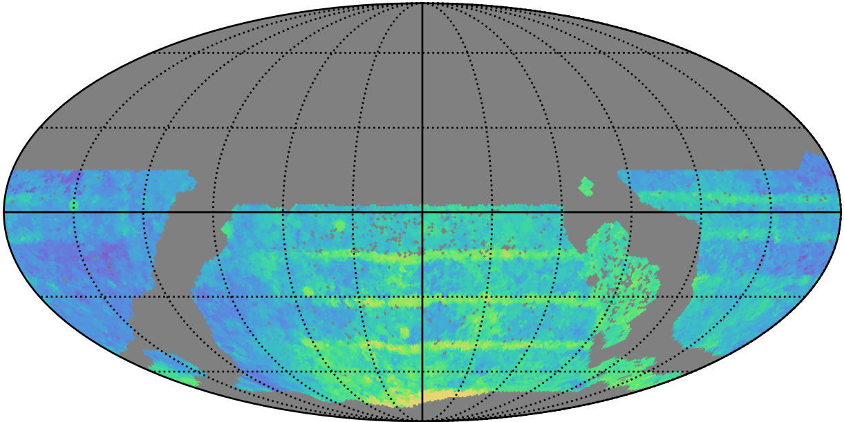
too_elab_heavy_r64_d2_gz_v3.4_10yrs WFD all bands: Median Season Length
