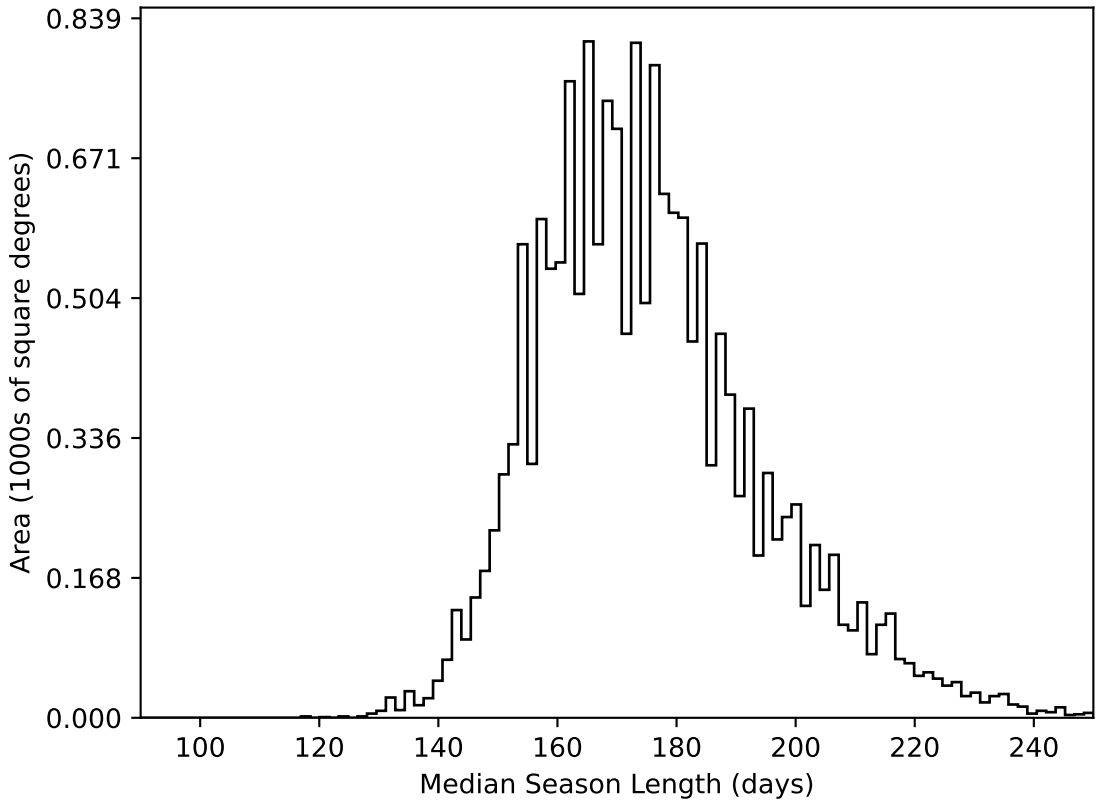
too_elab_heavy_r64_d2_gz_v3.4_10yrs WFD all bands: Median Season Length
