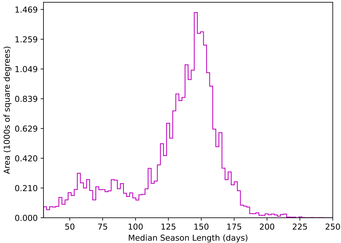
too_elab_heavy_r64_d2_gz_v3.4_10yrs All sky z band: Median Season Length
