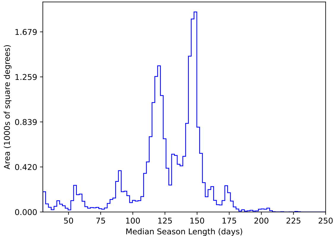
too_elab_heavy_r64_d2_gz_v3.4_10yrs All sky y band: Median Season Length
