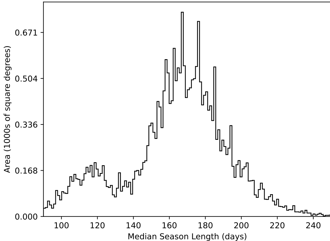
too_elab_heavy_r64_d2_gz_v3.4_10yrs All sky all bands: Median Season Length
