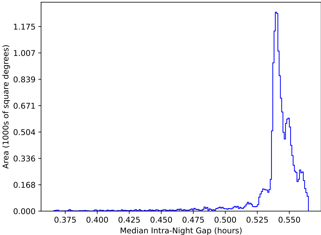
too_elab_heavy_r64_d2_gz_v3.4_10yrs WFD: Median Intra-Night Gap
