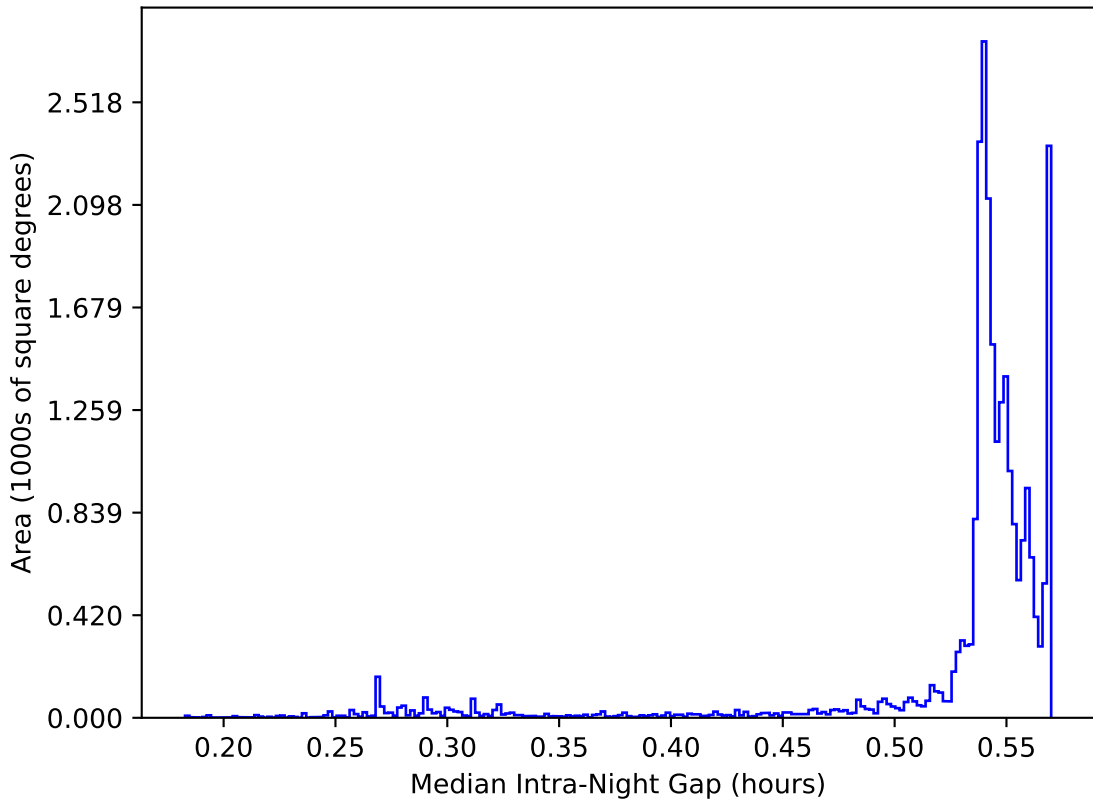
too_elab_heavy_r64_d2_gz_v3.4_10yrs All sky: Median Intra-Night Gap
