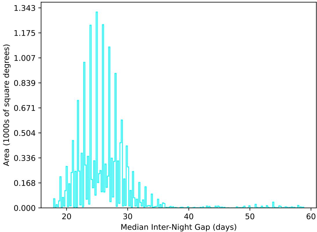
too_elab_heavy_r64_d2_gz_v3.4_10yrs WFD u band: Median Inter-Night Gap
