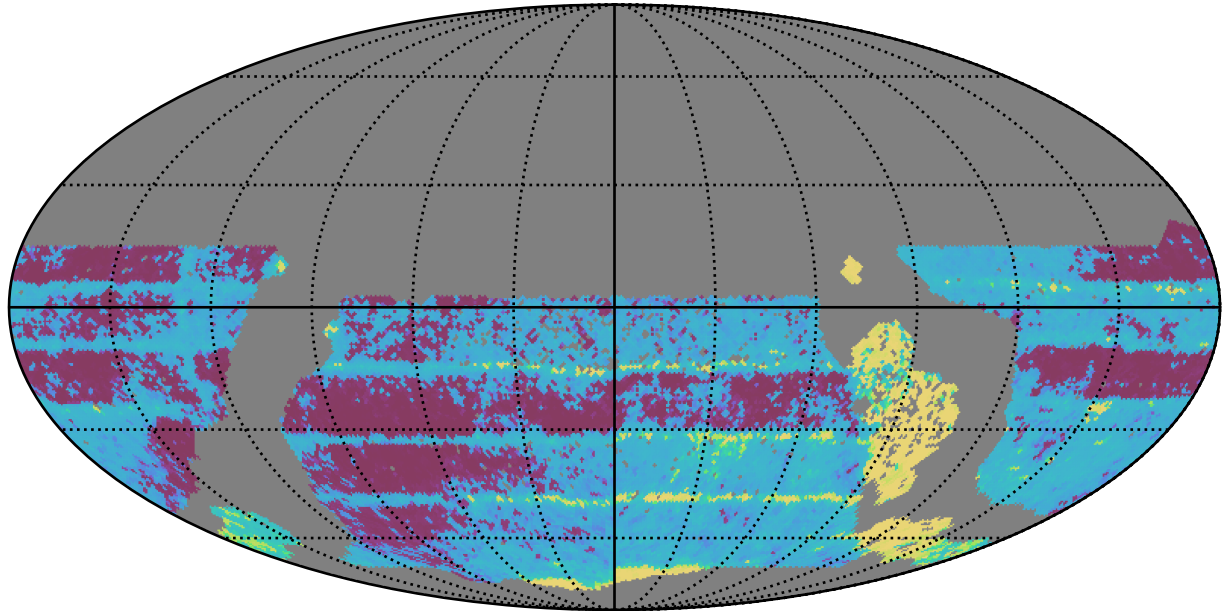
too_elab_heavy_r64_d2_gz_v3.4_10yrs WFD all bands: Median Inter-Night Gap
