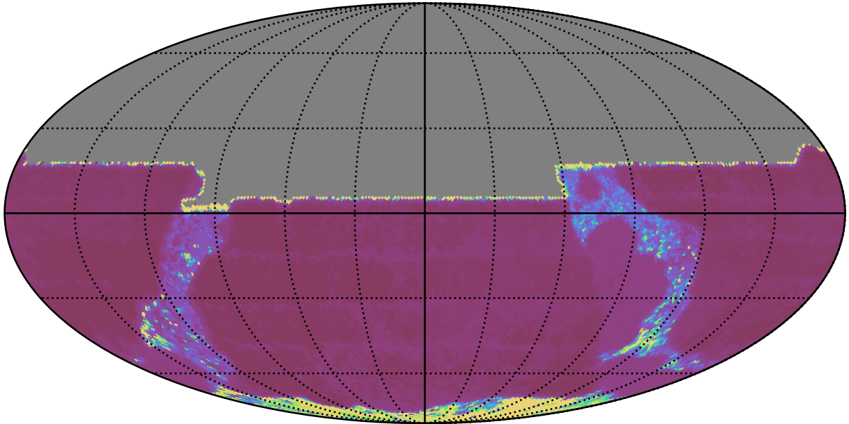
too_elab_heavy_r64_d2_gz_v3.4_10yrs All sky y band: Median Inter-Night Gap
