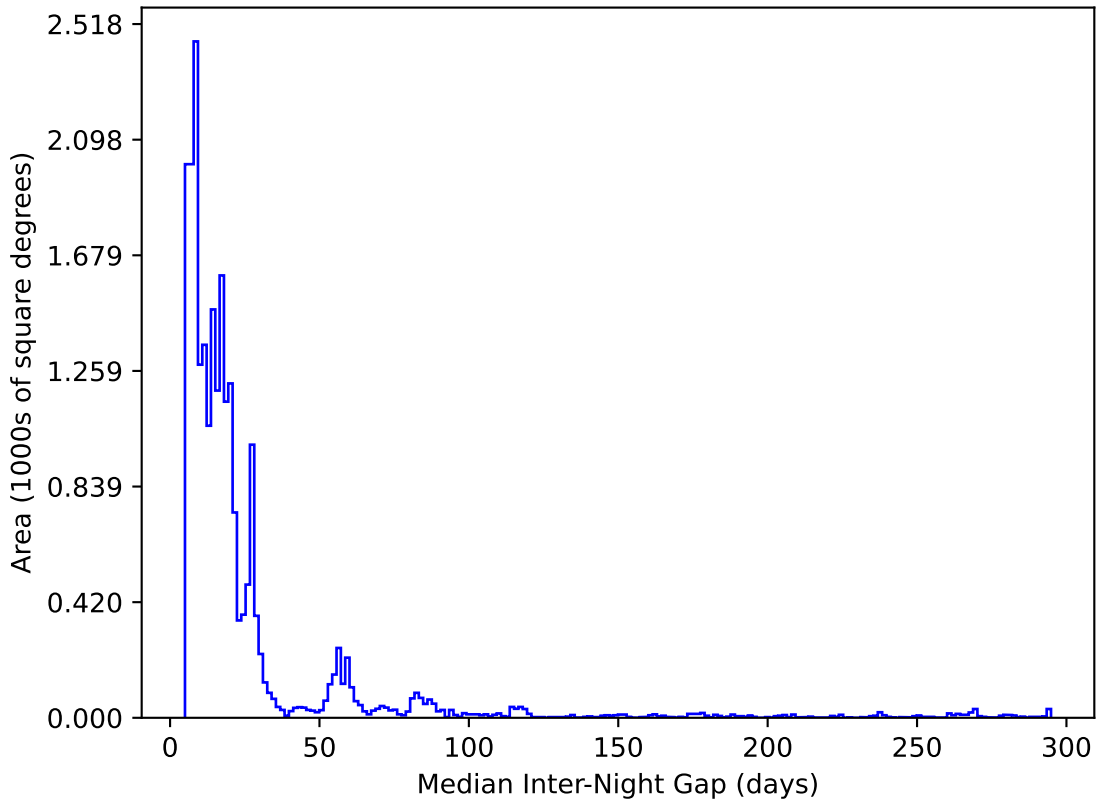
too_elab_heavy_r64_d2_gz_v3.4_10yrs All sky y band: Median Inter-Night Gap
