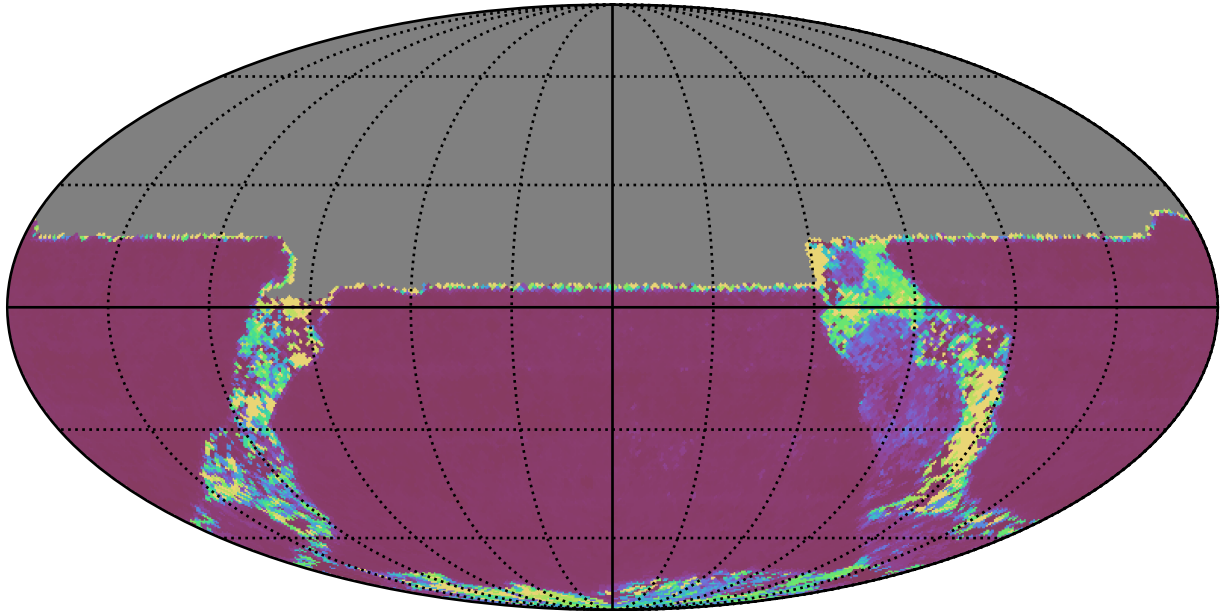
too_elab_heavy_r64_d2_gz_v3.4_10yrs All sky u band: Median Inter-Night Gap
