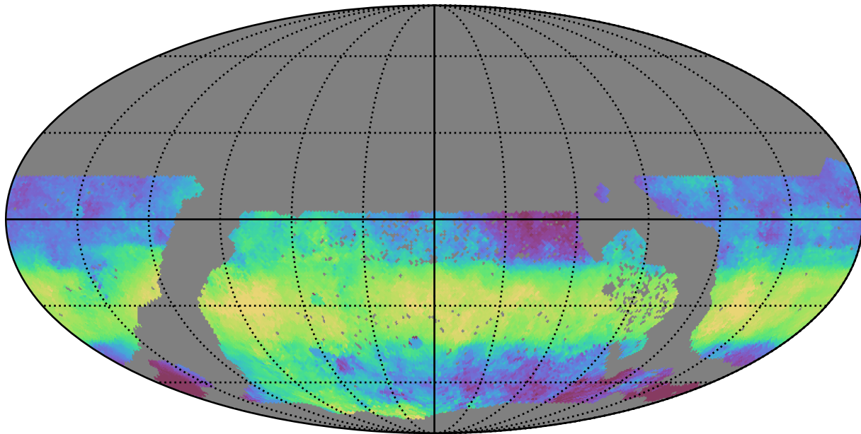
too_elab_heavy_r64_d2_gz_v3.4_10yrs WFD z band: Median HA
