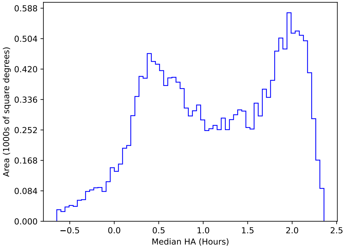
too_elab_heavy_r64_d2_gz_v3.4_10yrs WFD z band: Median HA
