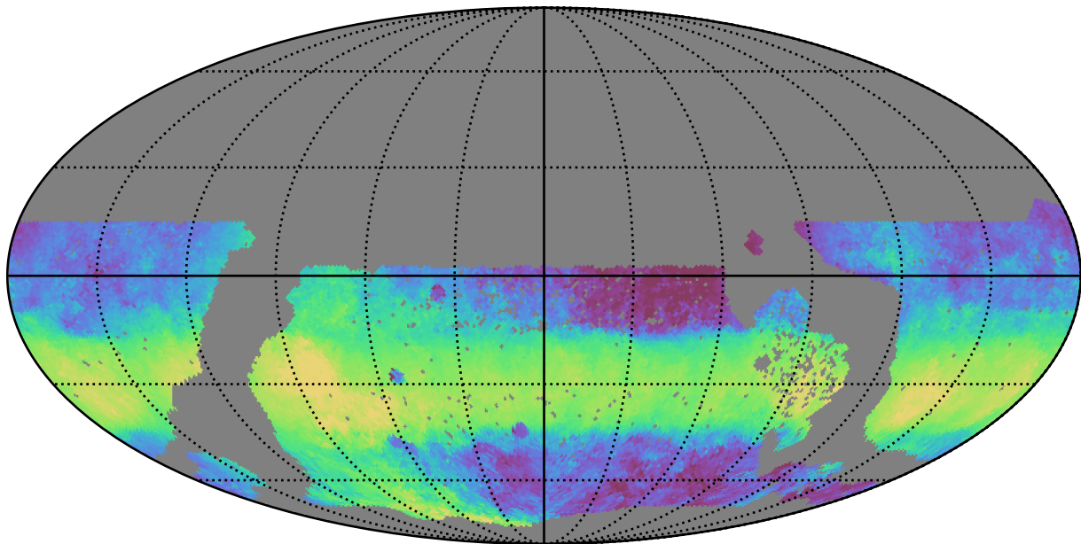
too_elab_heavy_r64_d2_gz_v3.4_10yrs WFD y band: Median HA
