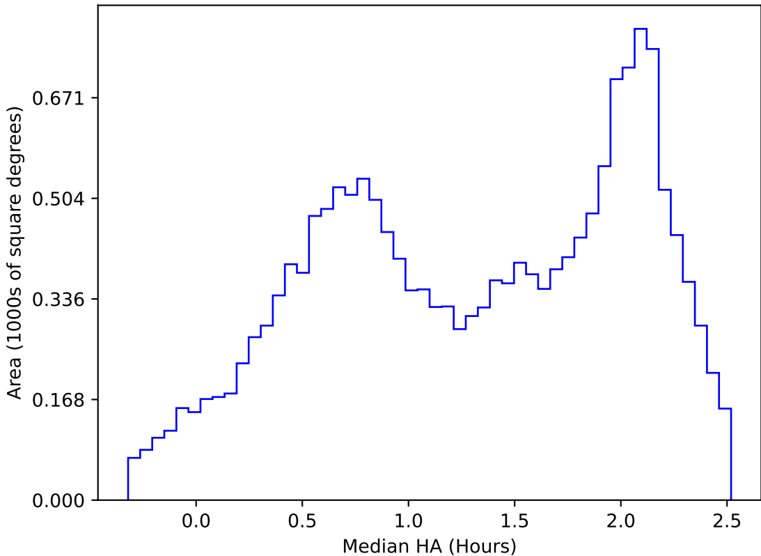
too_elab_heavy_r64_d2_gz_v3.4_10yrs WFD y band: Median HA
