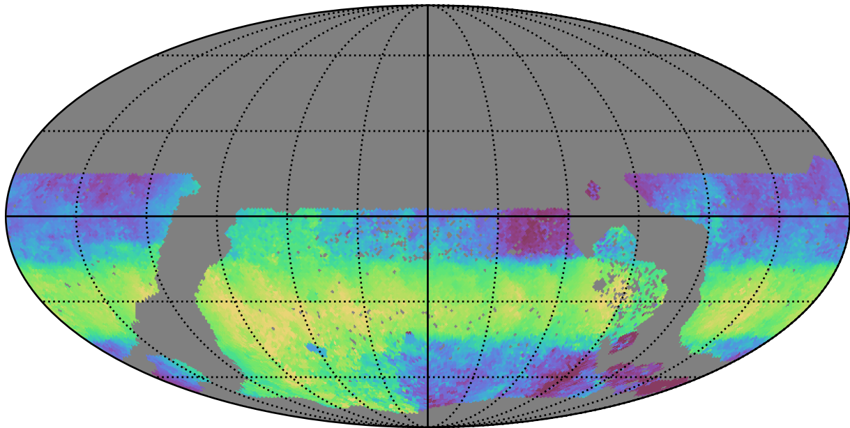
too_elab_heavy_r64_d2_gz_v3.4_10yrs WFD u band: Median HA
