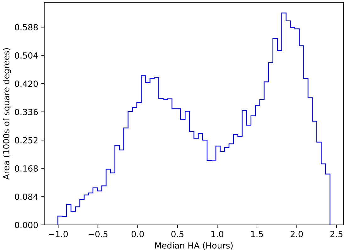
too_elab_heavy_r64_d2_gz_v3.4_10yrs WFD u band: Median HA
