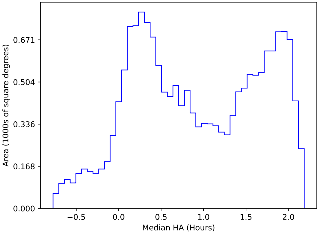
too_elab_heavy_r64_d2_gz_v3.4_10yrs WFD r band: Median HA
