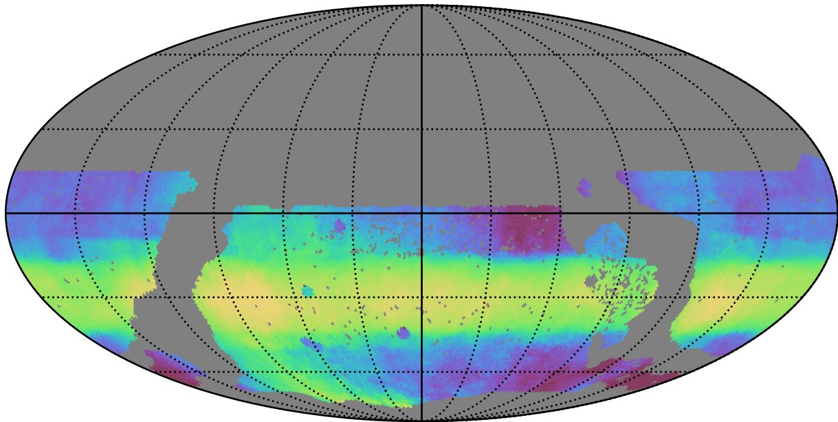
too_elab_heavy_r64_d2_gz_v3.4_10yrs WFD all bands: Median HA
