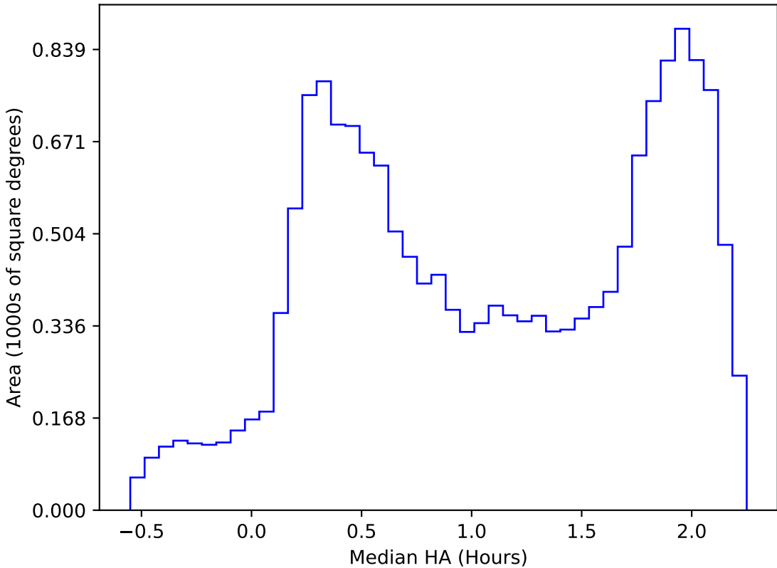
too_elab_heavy_r64_d2_gz_v3.4_10yrs WFD all bands: Median HA
