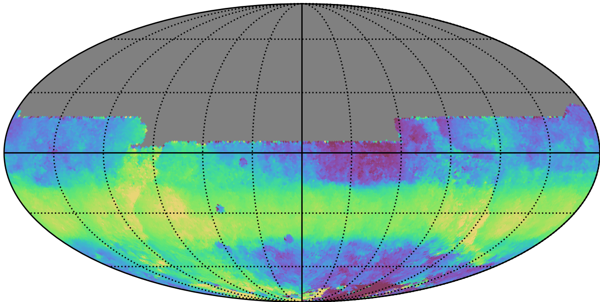
too_elab_heavy_r64_d2_gz_v3.4_10yrs All sky y band: Median HA
