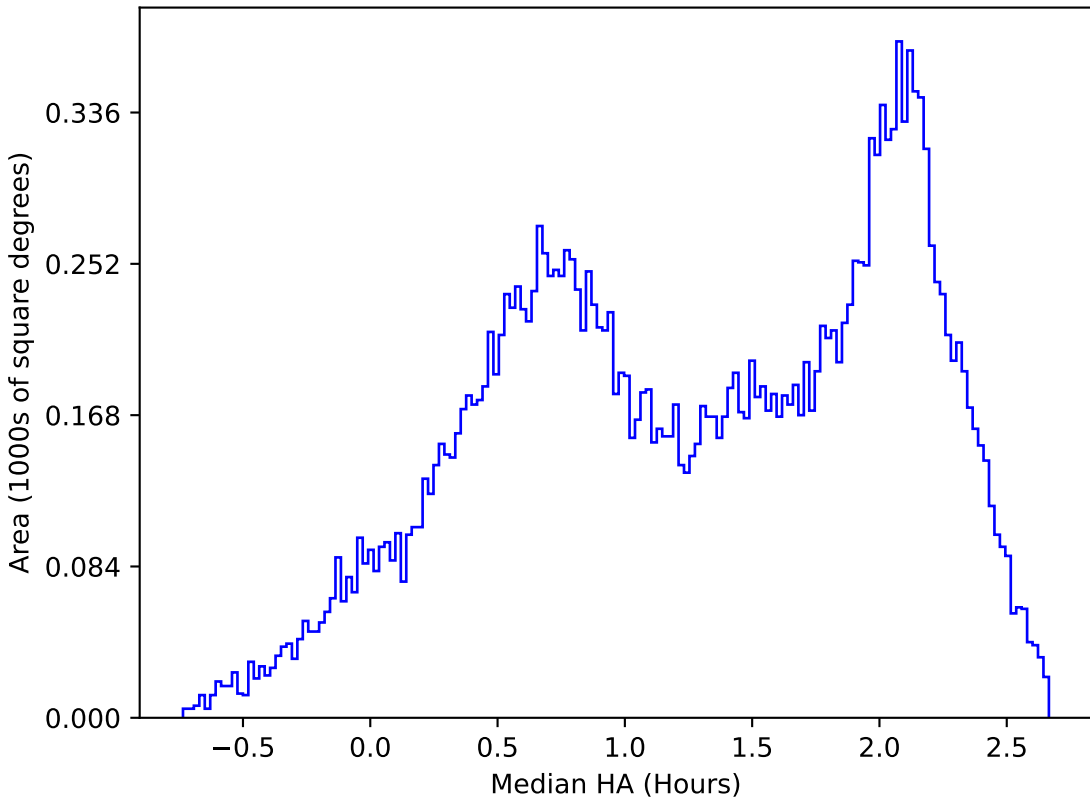
too_elab_heavy_r64_d2_gz_v3.4_10yrs All sky y band: Median HA
