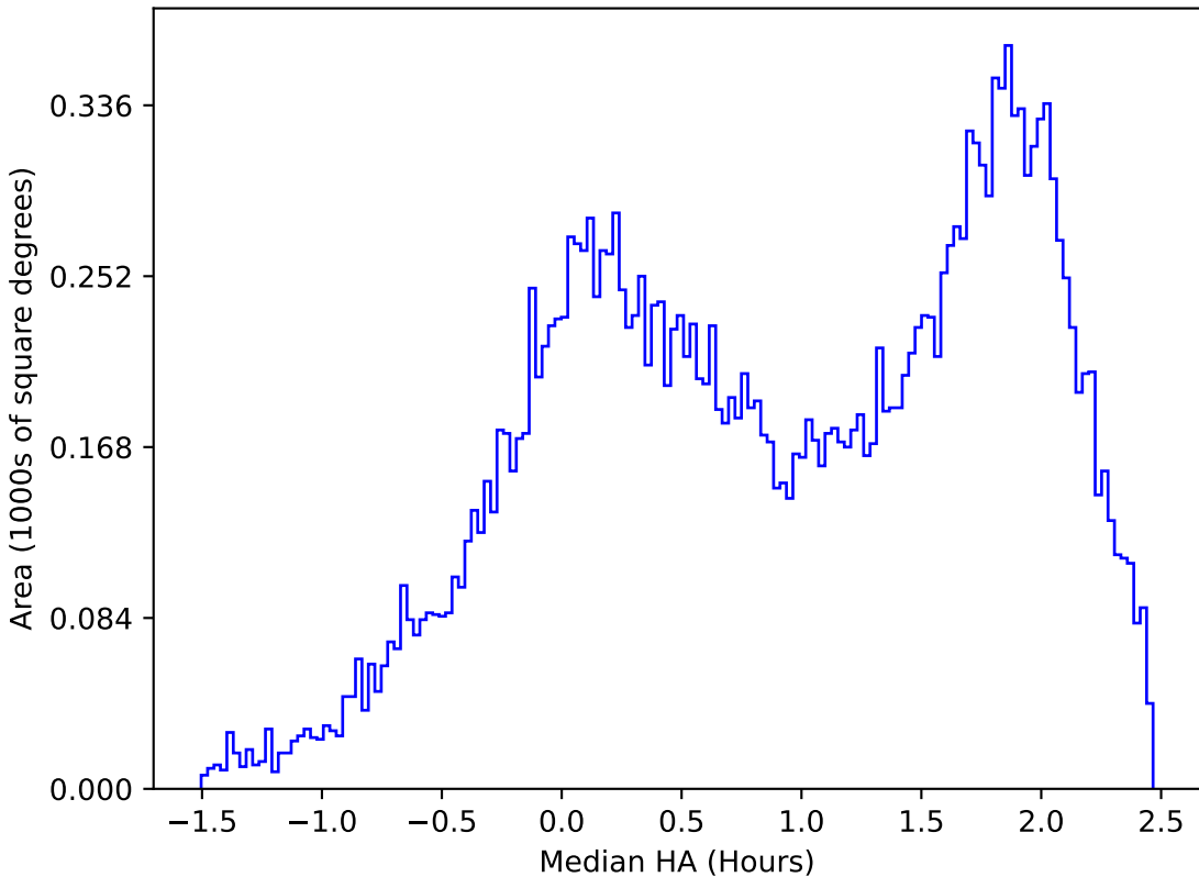
too_elab_heavy_r64_d2_gz_v3.4_10yrs All sky u band: Median HA
