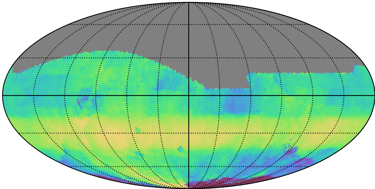
too_elab_heavy_r64_d2_gz_v3.4_10yrs All sky r band: Median HA
