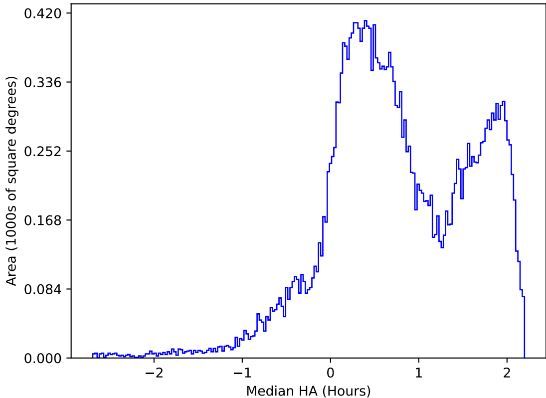
too_elab_heavy_r64_d2_gz_v3.4_10yrs All sky r band: Median HA
