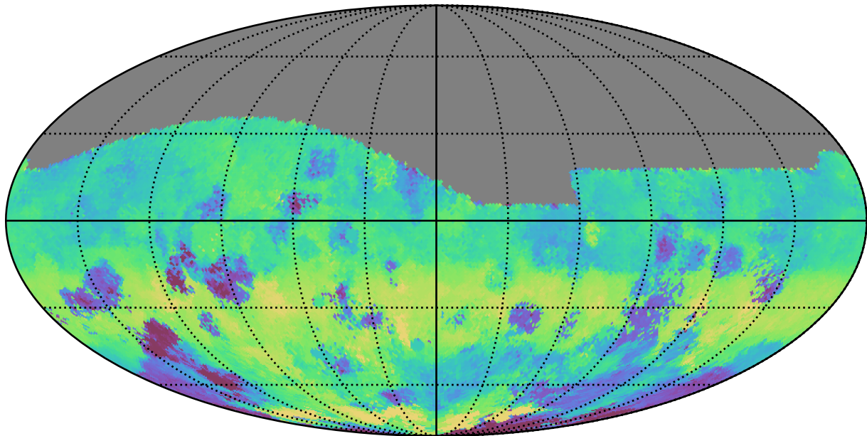
too_elab_heavy_r64_d2_gz_v3.4_10yrs All sky g band: Median HA
