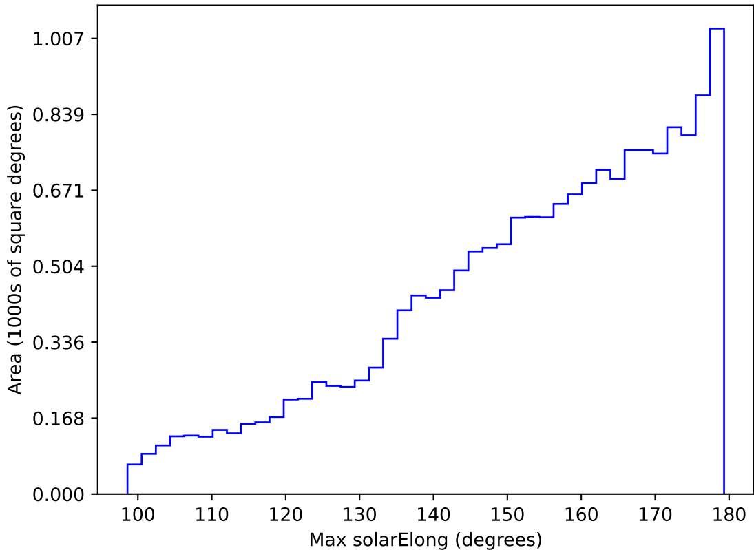
too_elab_heavy_r64_d2_gz_v3.4_10yrs WFD z band: Max solarElong
