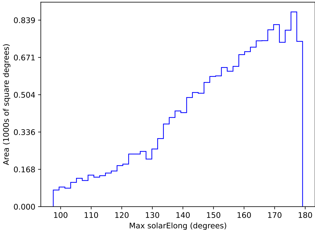
too_elab_heavy_r64_d2_gz_v3.4_10yrs WFD u band: Max solarElong
