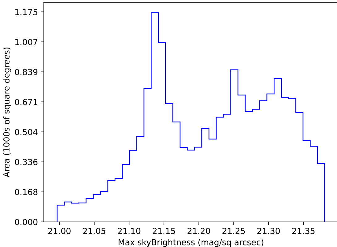
too_elab_heavy_r64_d2_gz_v3.4_10yrs WFD r band: Max skyBrightness
