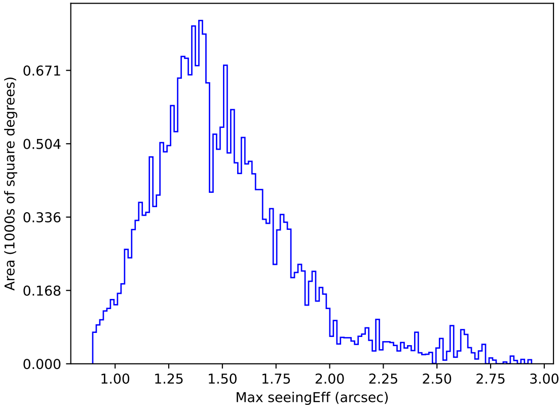
too_elab_heavy_r64_d2_gz_v3.4_10yrs Yr 1 z band: Max seeingEff
