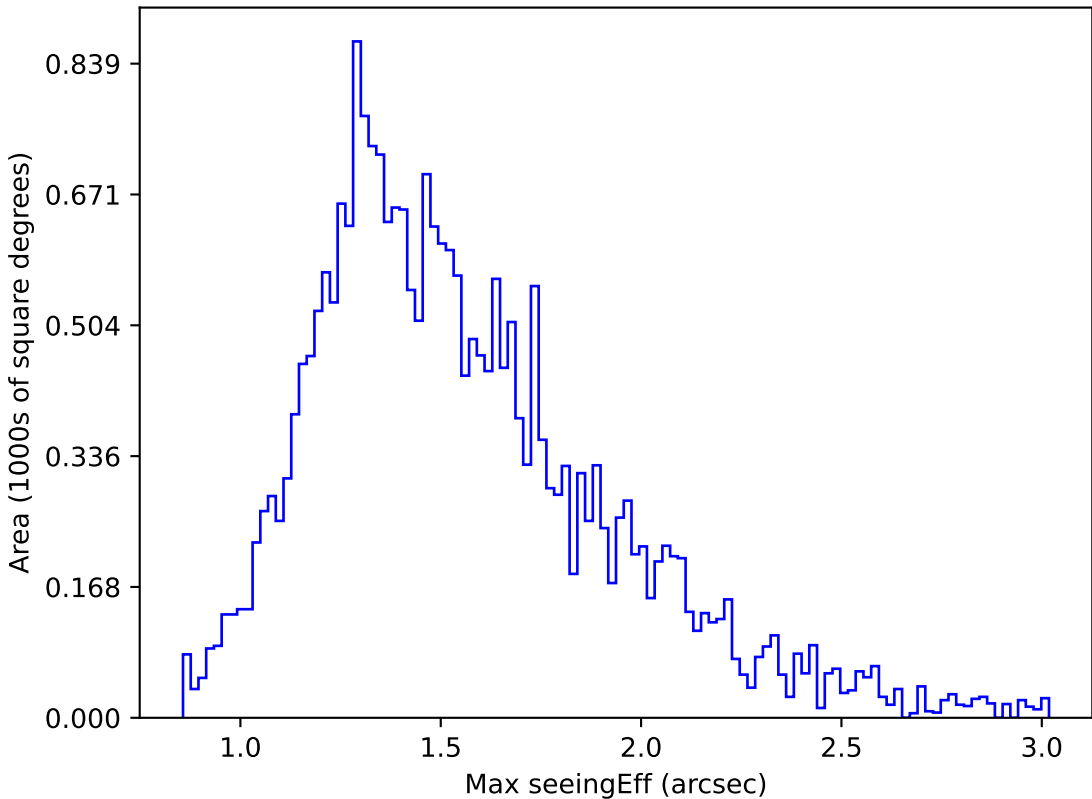
too_elab_heavy_r64_d2_gz_v3.4_10yrs Yr 1 g band: Max seeingEff
