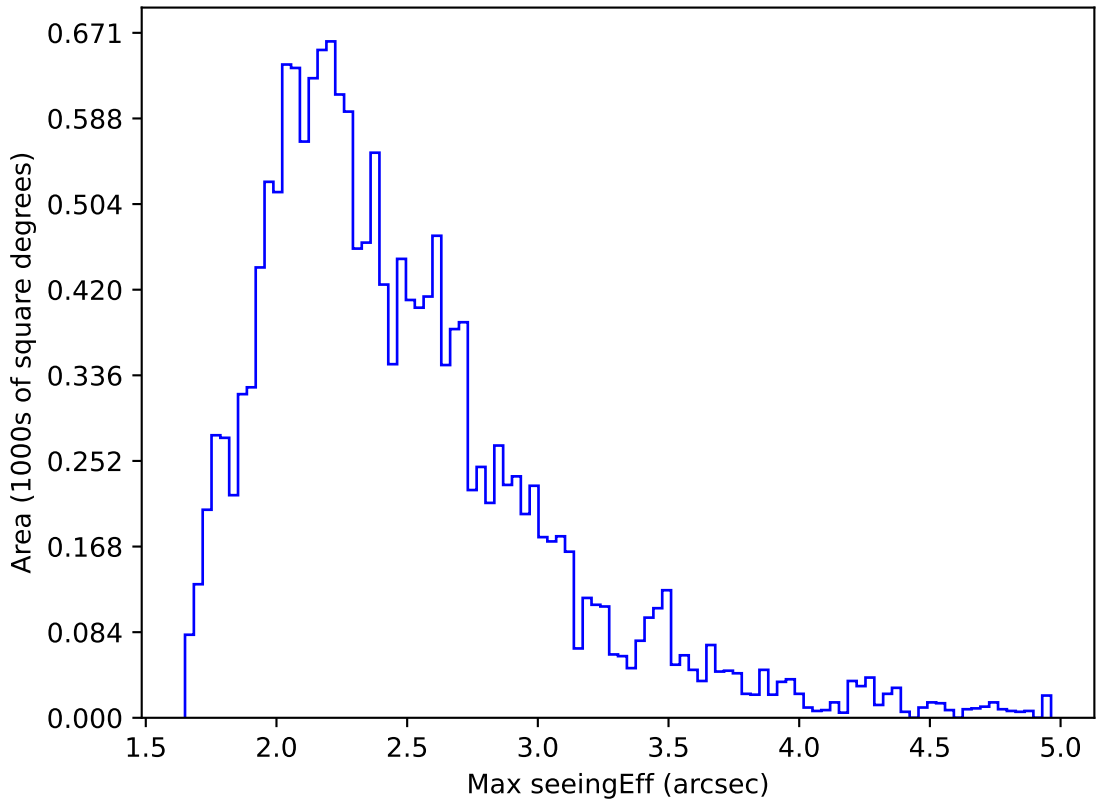
too_elab_heavy_r64_d2_gz_v3.4_10yrs WFD z band: Max seeingEff
