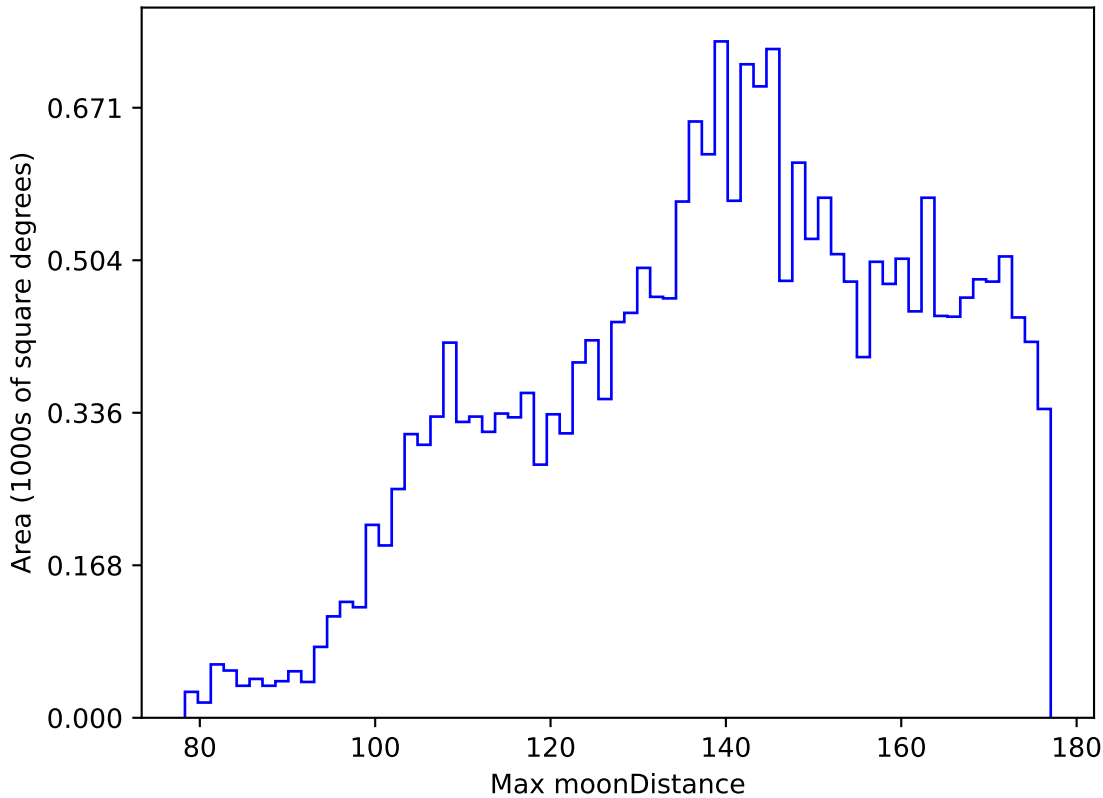
too_elab_heavy_r64_d2_gz_v3.4_10yrs All sky y band: Max moonDistance
