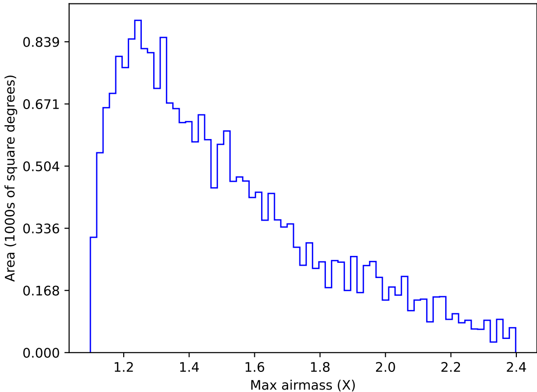
too_elab_heavy_r64_d2_gz_v3.4_10yrs Yr 1 u band: Max airmass
