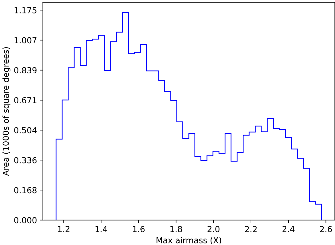
too_elab_heavy_r64_d2_gz_v3.4_10yrs Yr 1 r band: Max airmass
