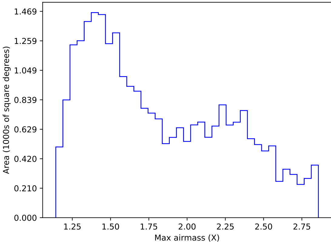
too_elab_heavy_r64_d2_gz_v3.4_10yrs Yr 1 i band: Max airmass
